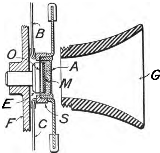
FIG. 74.—Telephone transmitter.
